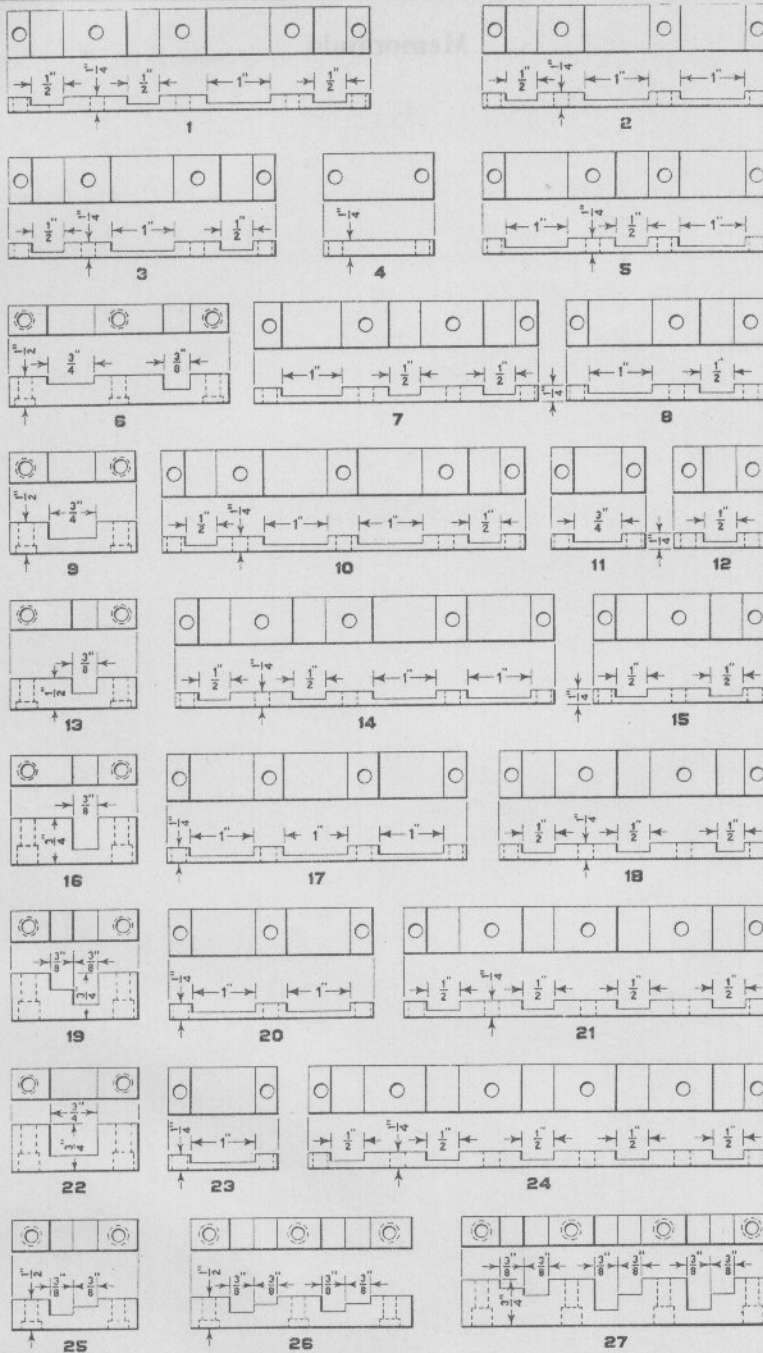
Locking Bar Guides For Model 2 Electric Interlocking Machines
