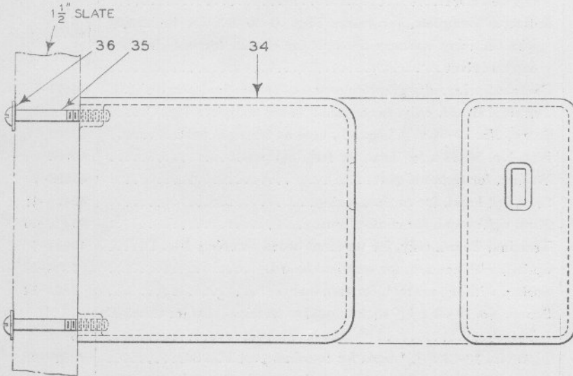
C - Cover Polarized Relays For Switchboards
